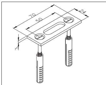
Art. No. 1-228 Schließblech aus Niro, mit Holzschrauben DIN 97, 6 x 50 mm und Kunststoffdübel S8 Art. No. 1-228 Locking plate made from stainless steel, with slotted countersunk head wood screw 6 x 50 mm with plastic dowel S8
