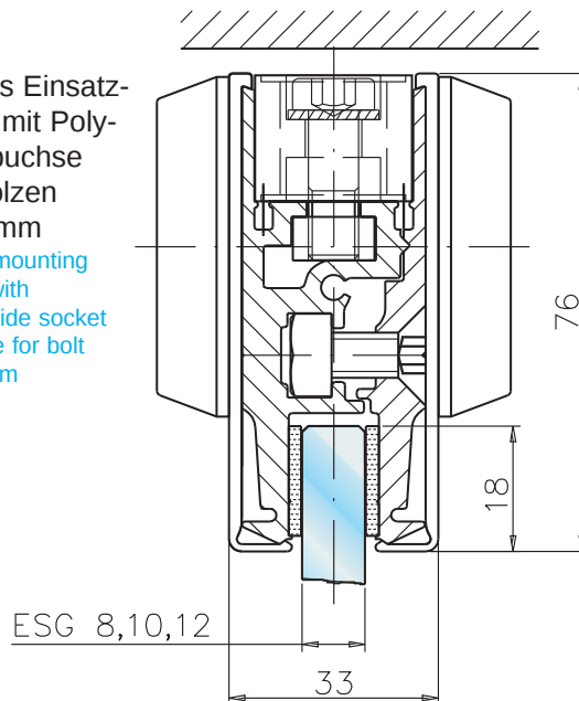
Art. No. 2-702
