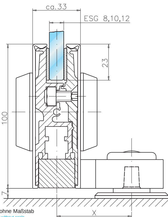
Art. No. 2-108
