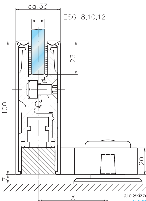
Art. No. 2-106
